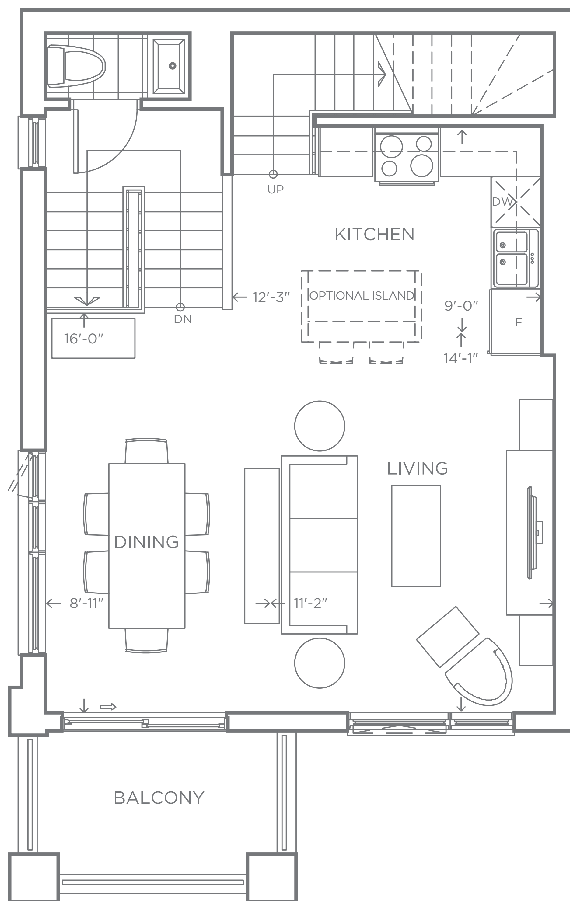
SECOND FLOOR
