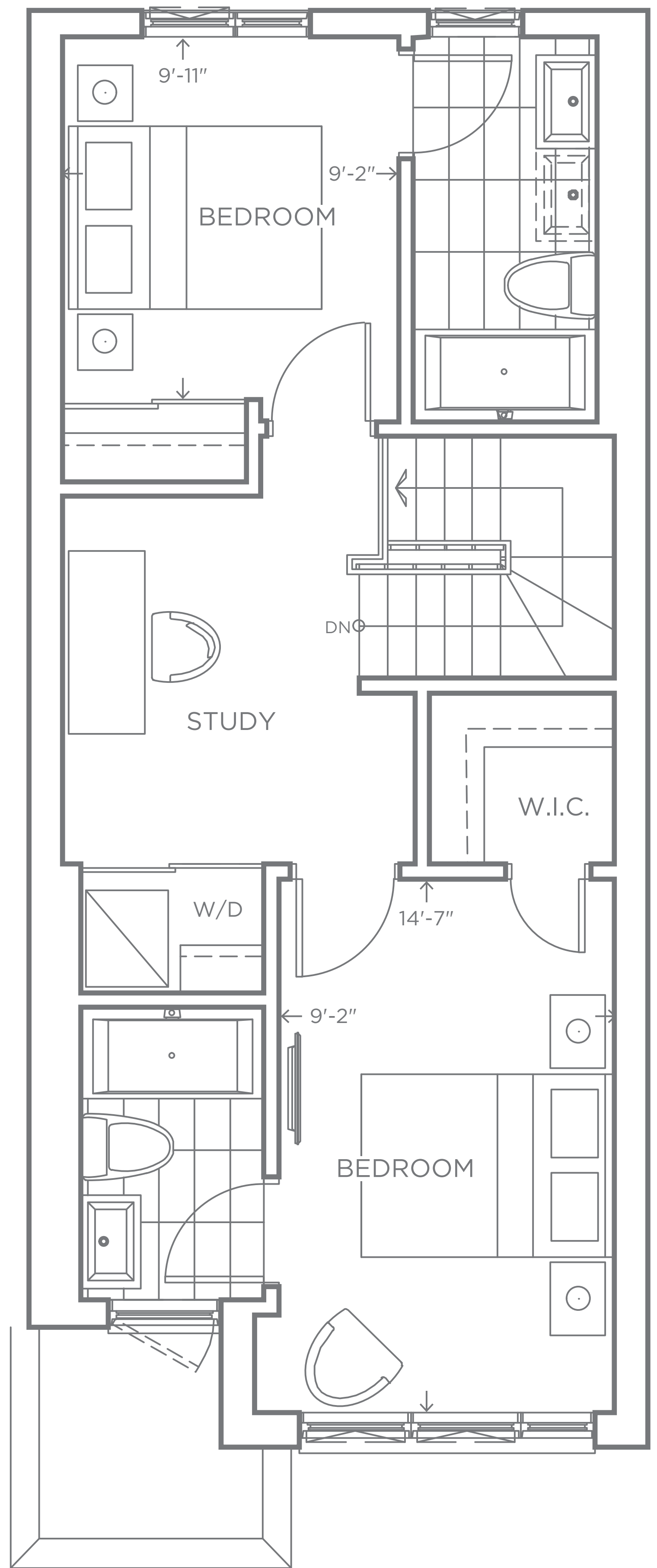
THIRD FLOOR
