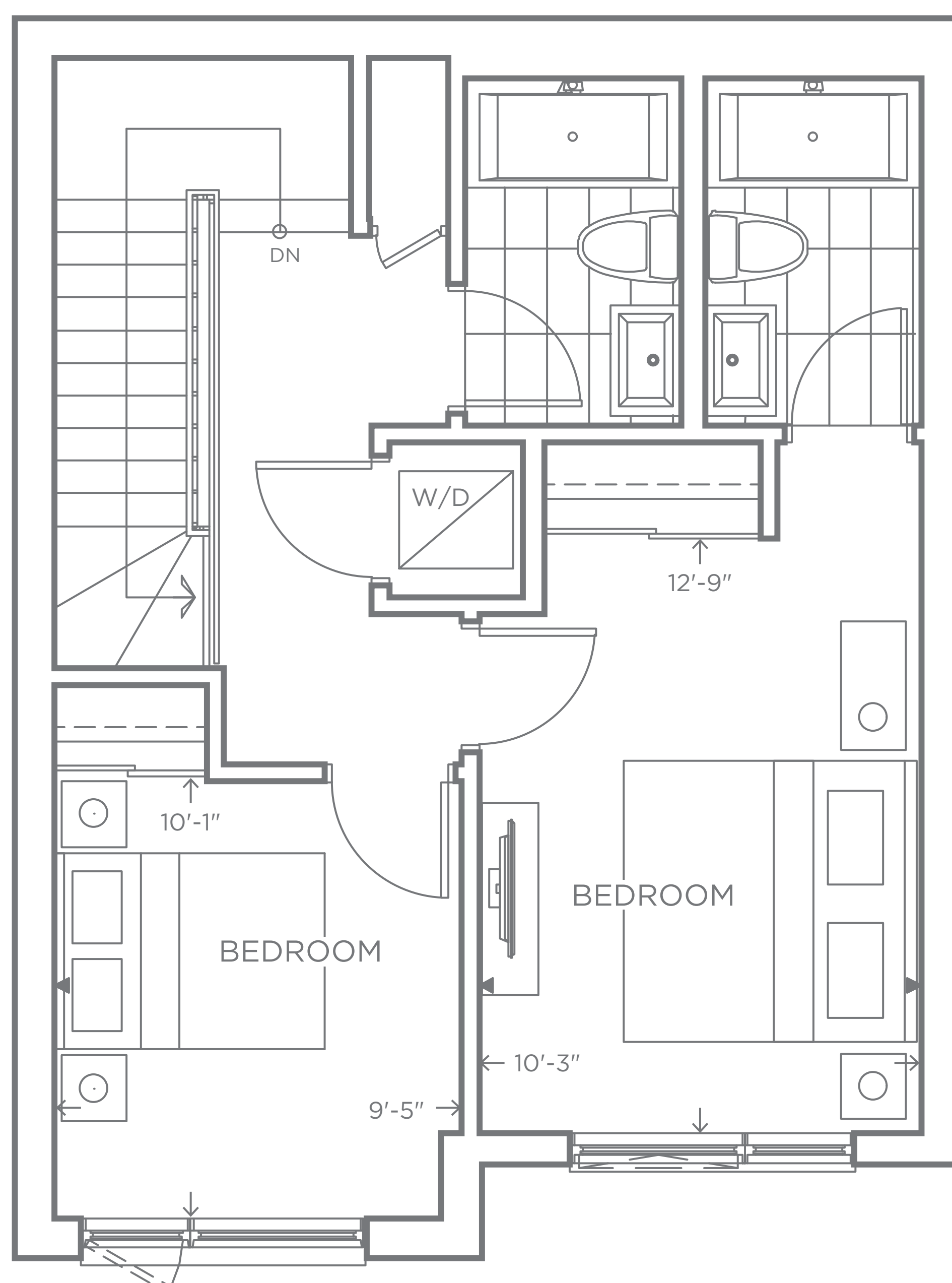
THIRD FLOOR
