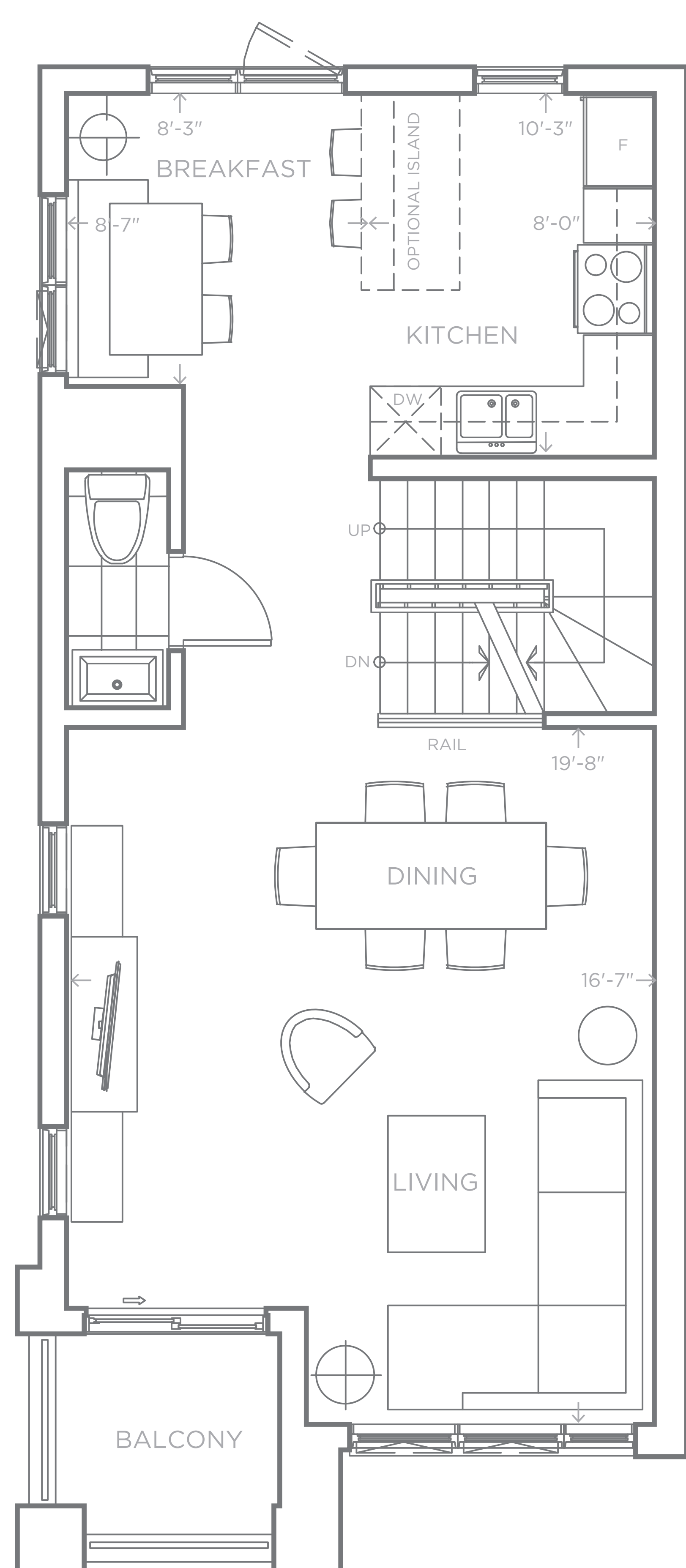
SECOND FLOOR
