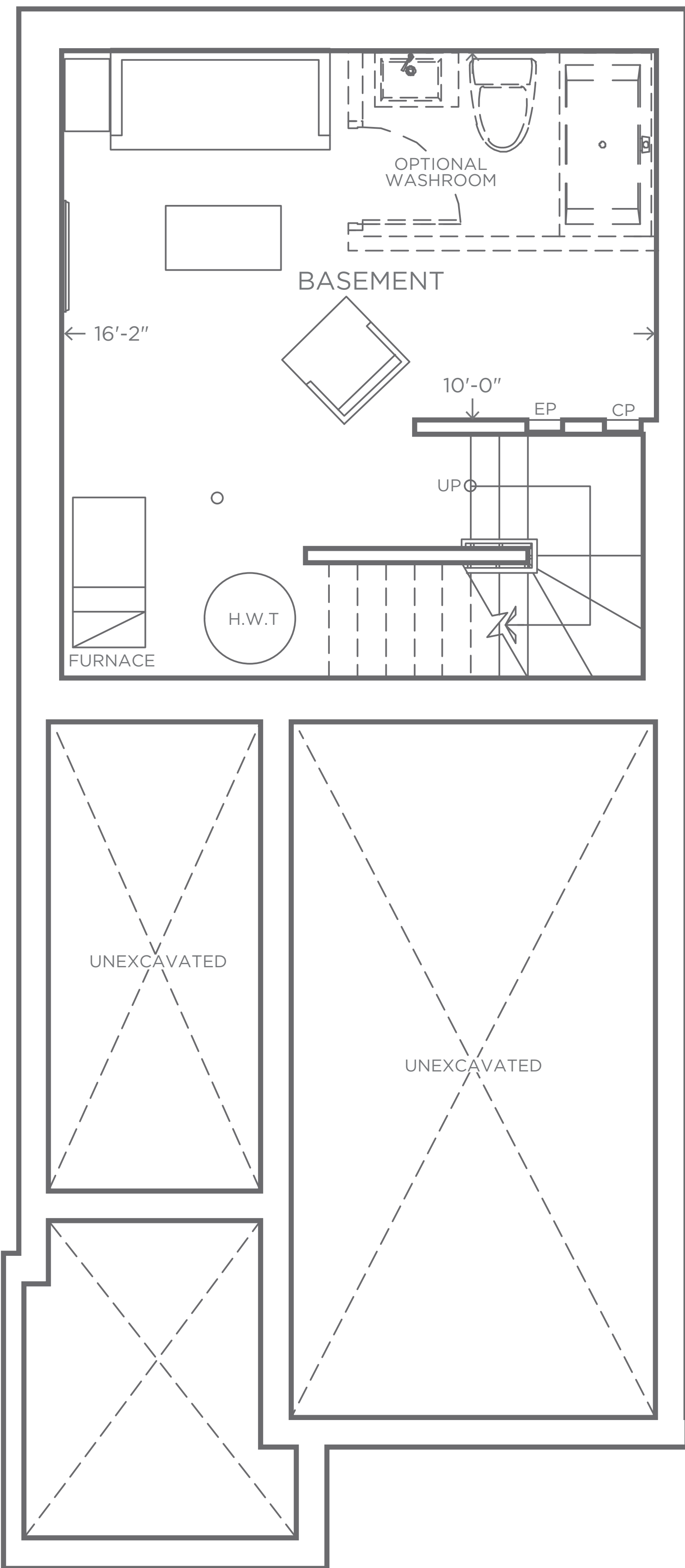
BASEMENT
