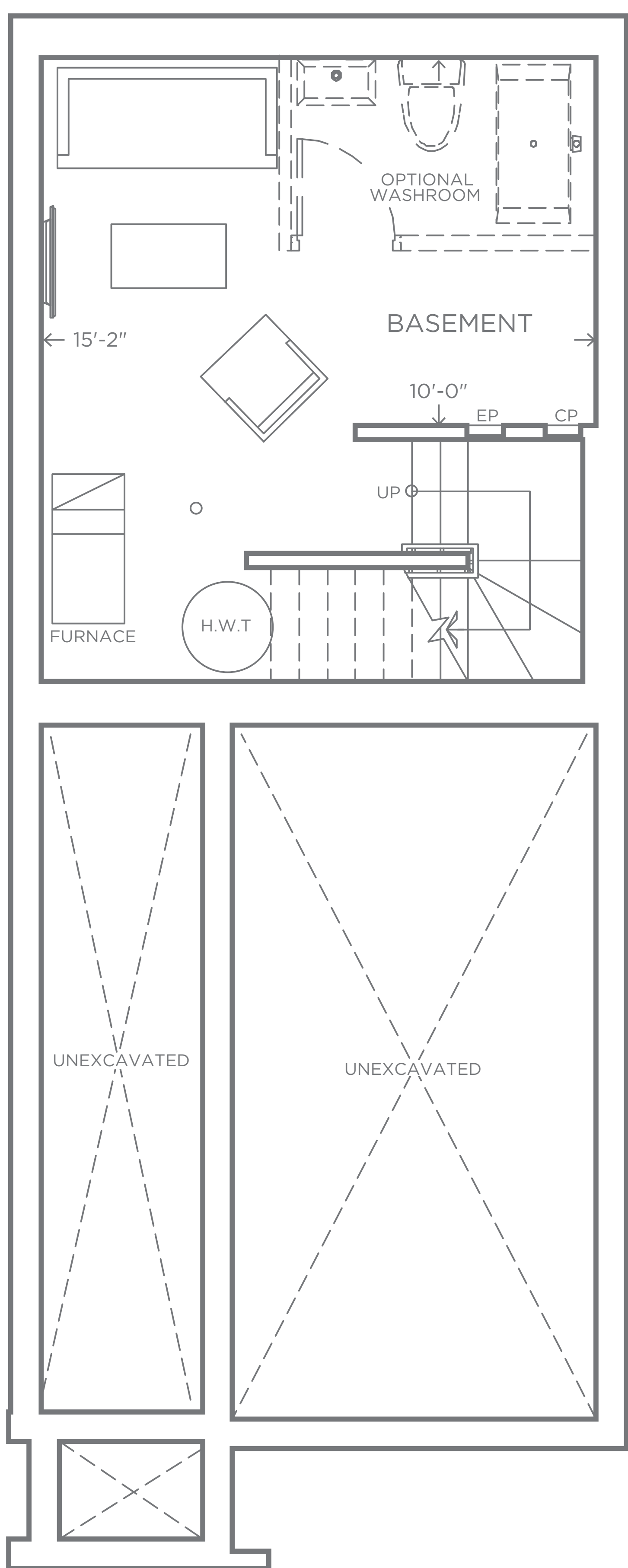
BASEMENT
