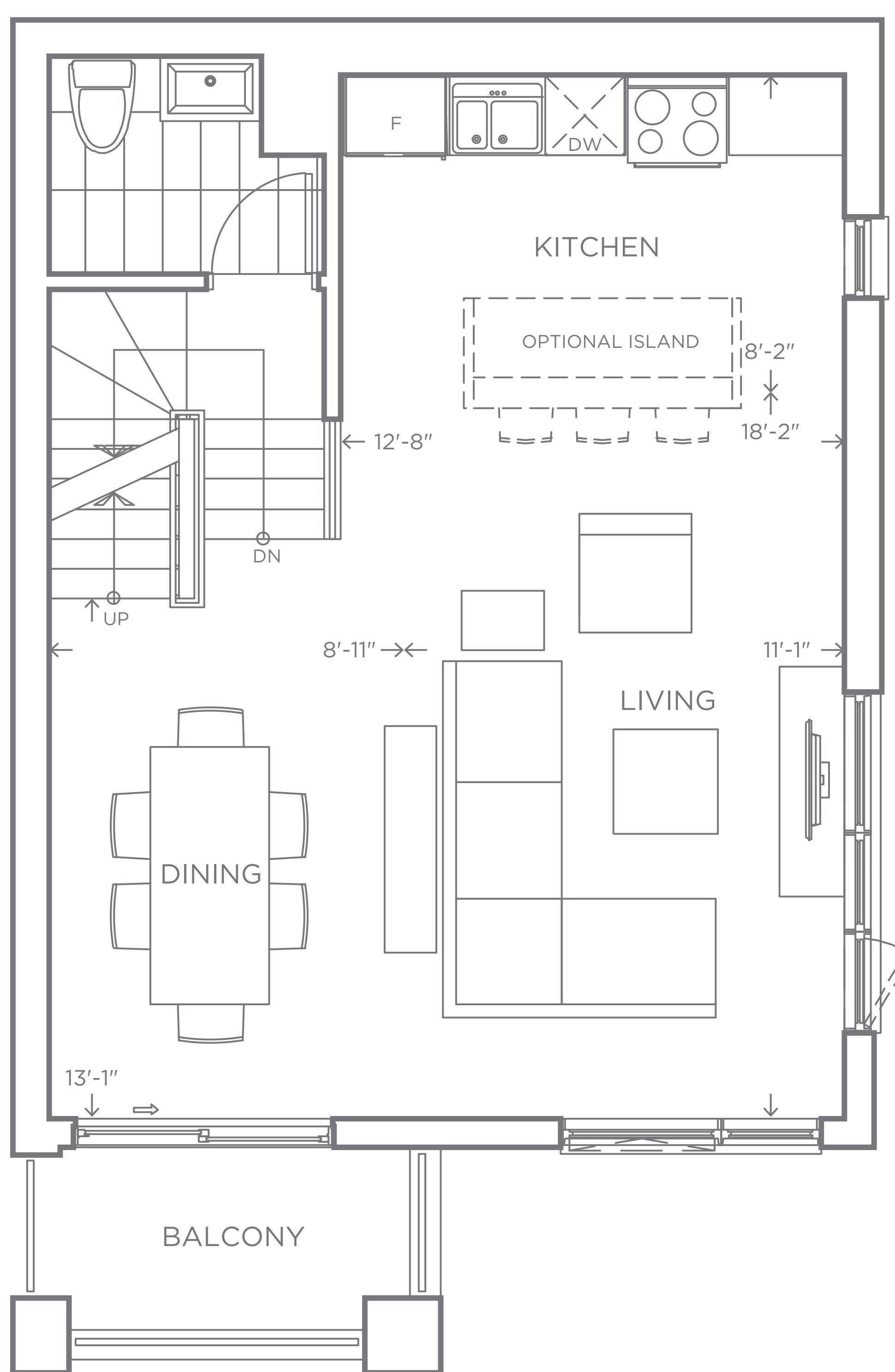
SECOND FLOOR
