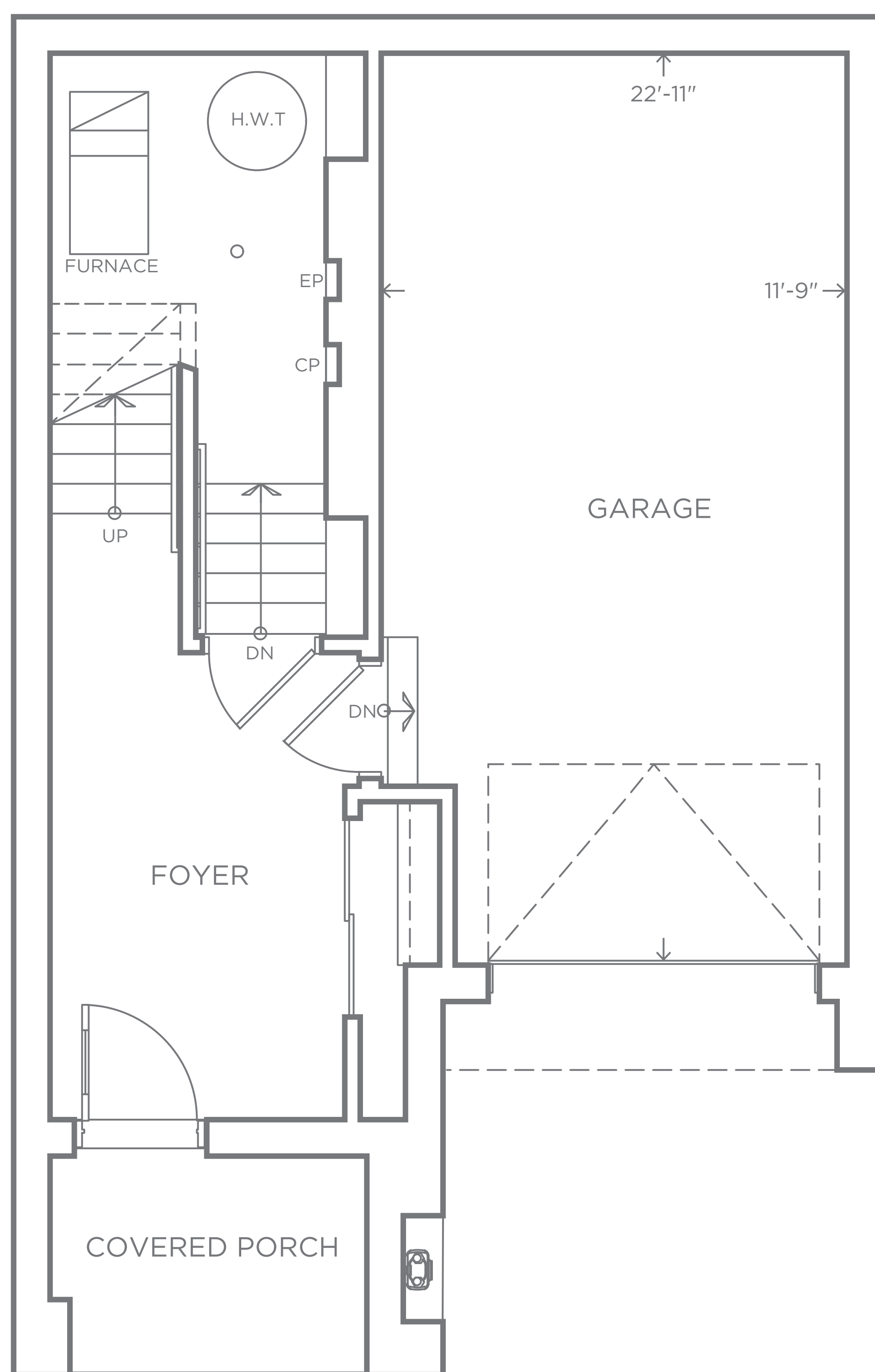
GROUND FLOOR
