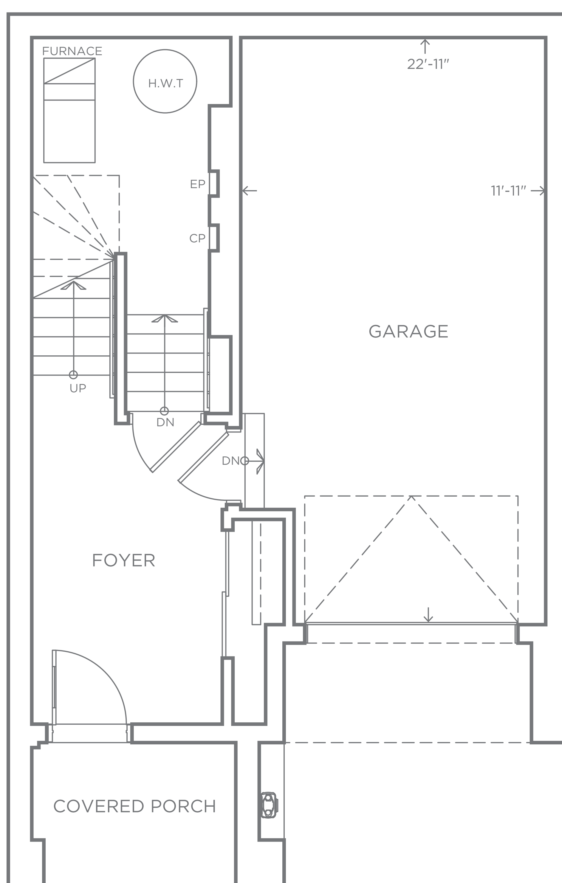
GROUND FLOOR
